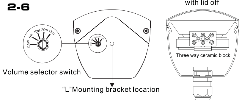
Top View of Column Loudspeaker with lid off
